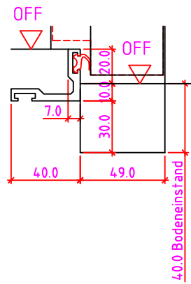
30mm Winkelschiene
