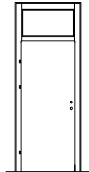
RST-K Anschlag links
