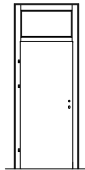
RST-K Anschlag links
