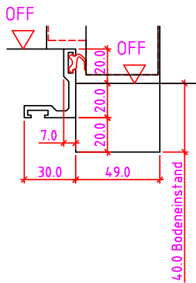
40mm Winkelschiene
