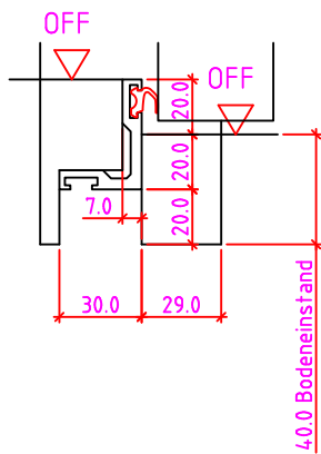
40mm Winkelschiene
