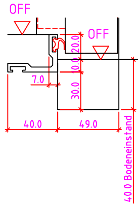
30mm Winkelschiene
