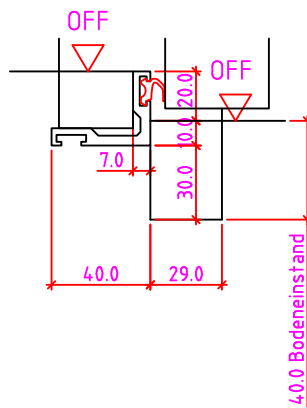
30mm Winkelschiene
