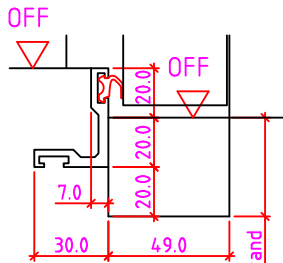
40mm Winkelschiene
