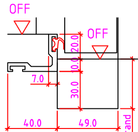
30mm Winkelschiene
