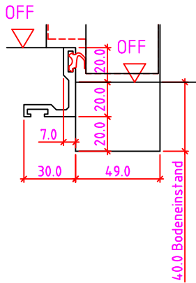
40mm Winkelschiene
